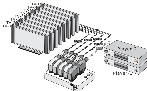
SB-3722 SCART DISTRIBUTION AMPLIFIER 2x1x8
